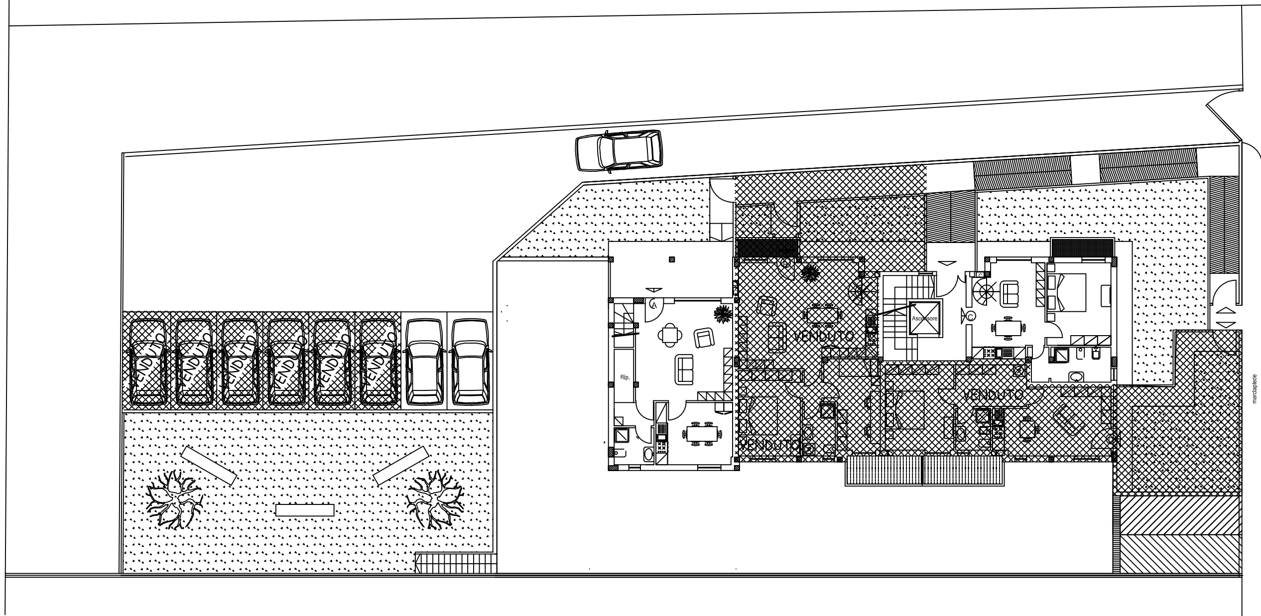
Piano terra
